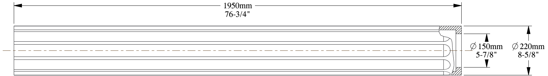
SECTION A-A SCALE 1:10
